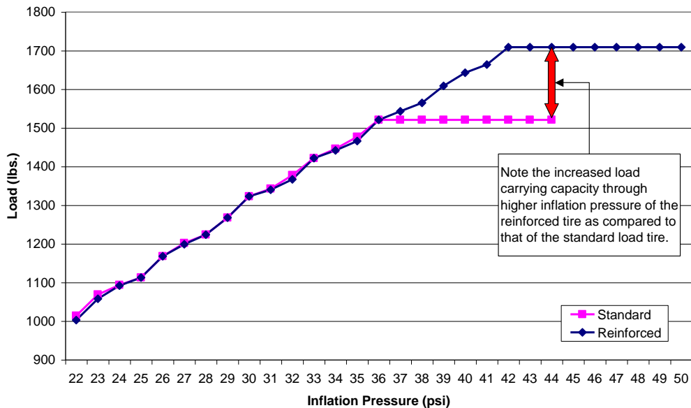
Figure 2. ETRTO example of 225/50R16 Standard Load vs. Reinforced/Extra Load.
